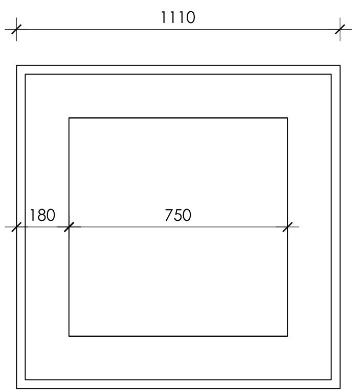
PROFILE 1 - Square (750 internal)
