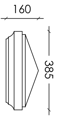
DEC 3 - Stepped Decorative
