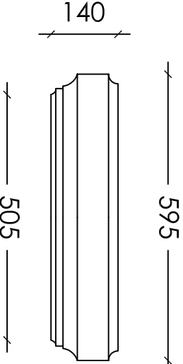
DEC 19 - Mandalay Pedestal Cap
