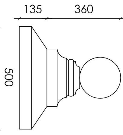
DEC 6 - Pyramid with ball & finial
