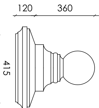
DEC 10 - Stepped Decorative with ball & finial
