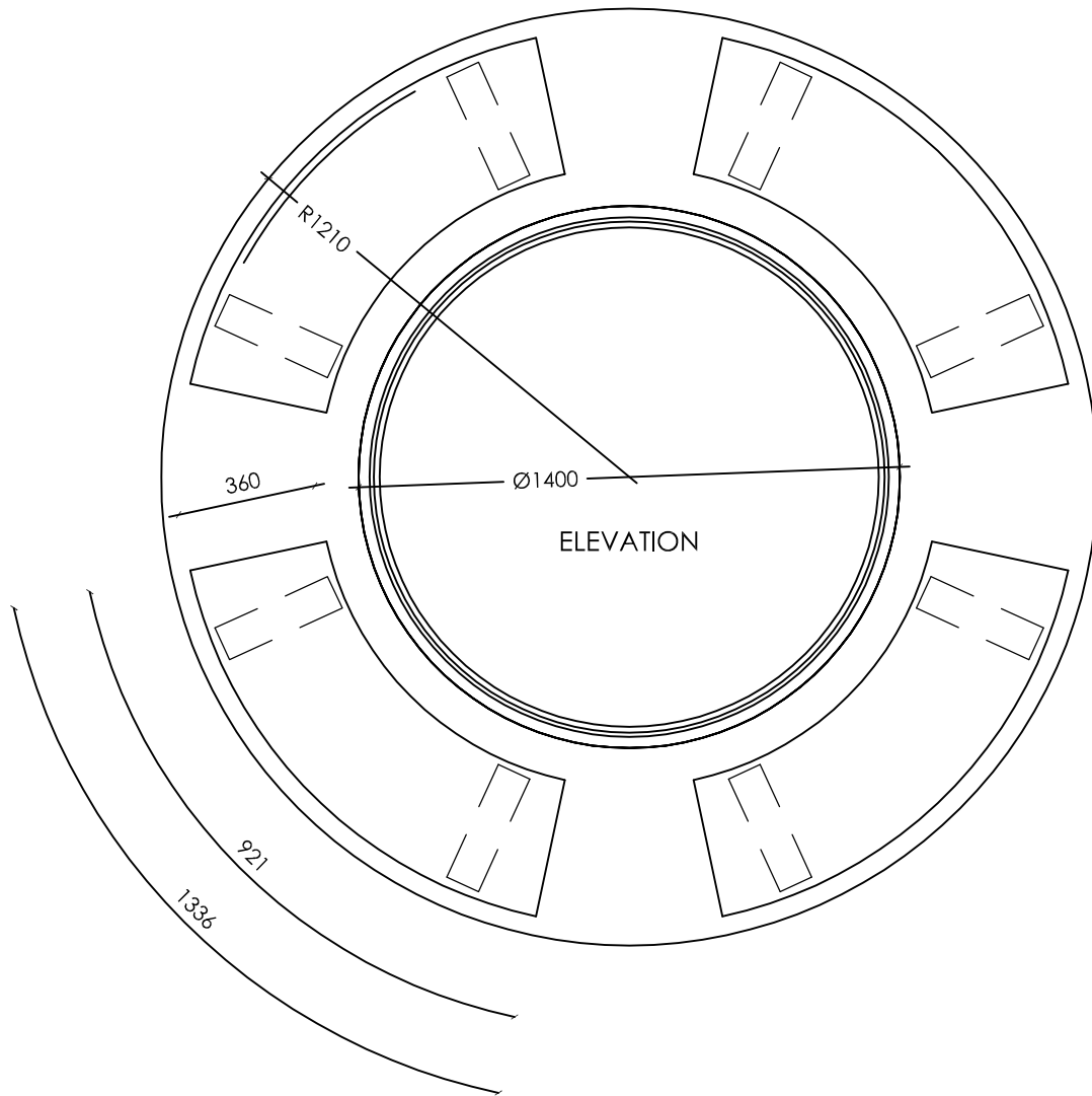
PLAN SETOUT - 1400 DIA. TABLE & 4 BENCH SEATS
