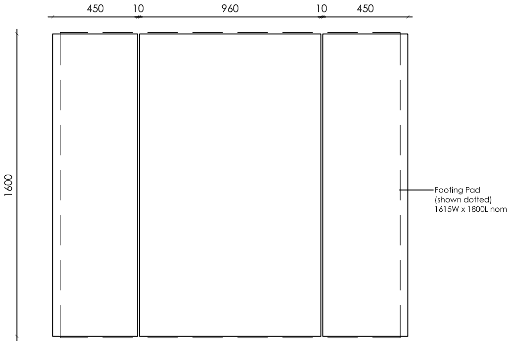
PLAN SETOUT - RECTANGULAR TABLE & 2 X BENCH SEATS
